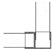
DS4/17 CORNER SECTION (OPTION)
