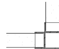
TWO WAY MULLION (corner)
