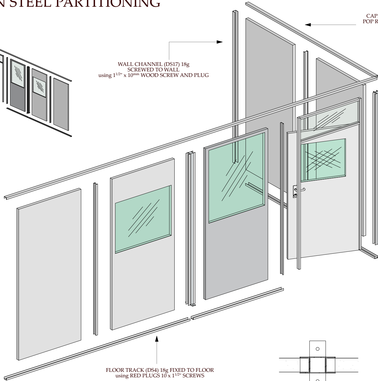
TWO WAY MULLION (inter)
