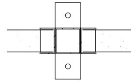
TWO WAY MULLION (inter)
